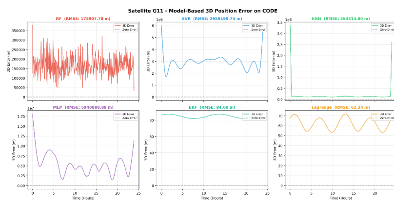
Figure 4. Model-Based 3D Position Error (LOO-CV) for CODE Analysis Center
